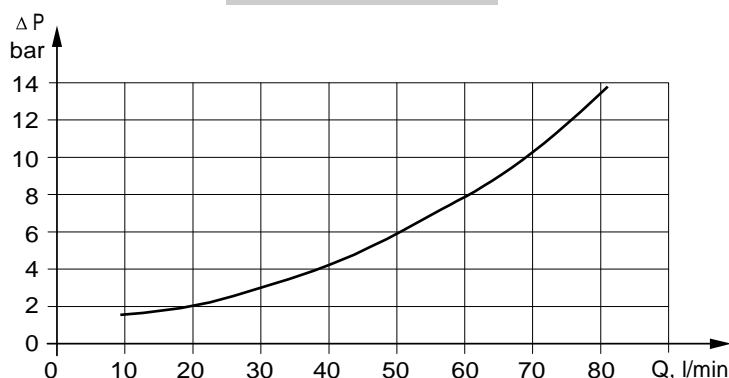
Pressure Losses
